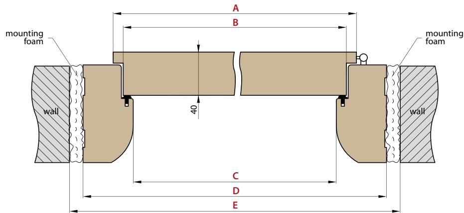
CROSS SECTION
